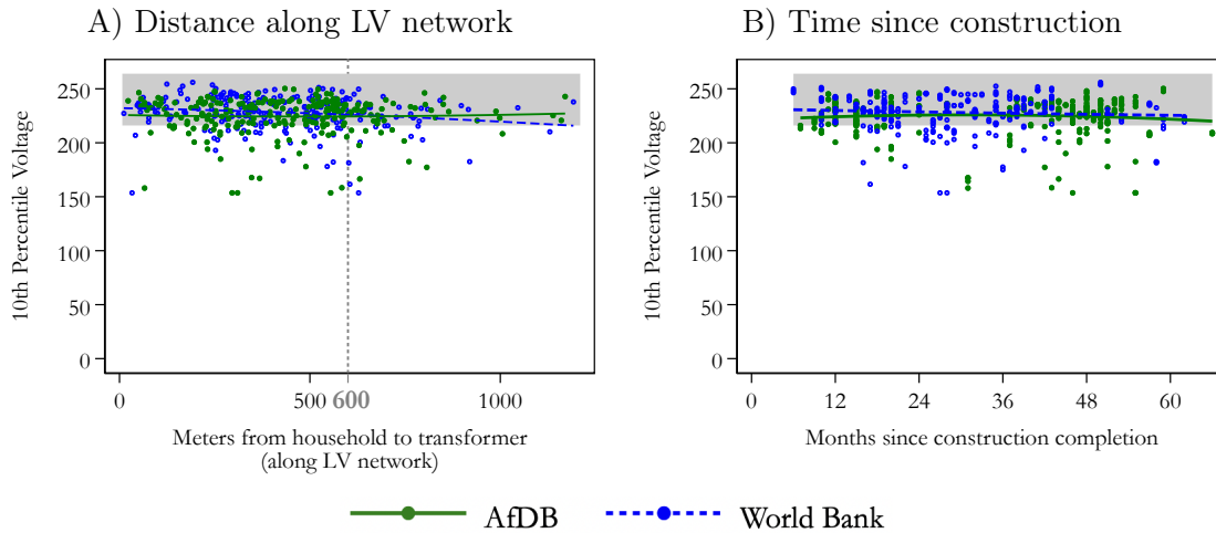
Figure A13: Voltage quality resilience to distance and infrastructure aging
